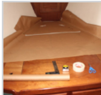
11 - Measure the Beveled Edge. Be sure to measure Bevel each Row of Paper & Work your Way off of the Platform. This way you don't have to crawl on top of the pattern and chance moving it around.
